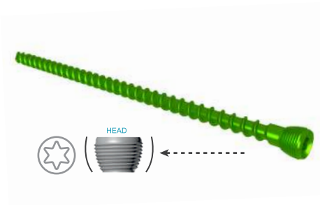
3.5 mm Variable Angle Cancellous Locking Head Screw [LHS] Star
